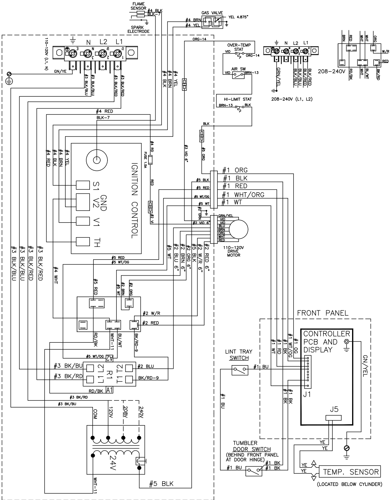
9506-821-001PR WIRING DIAGRAM DNS020N_-15_B_X-____-__X
