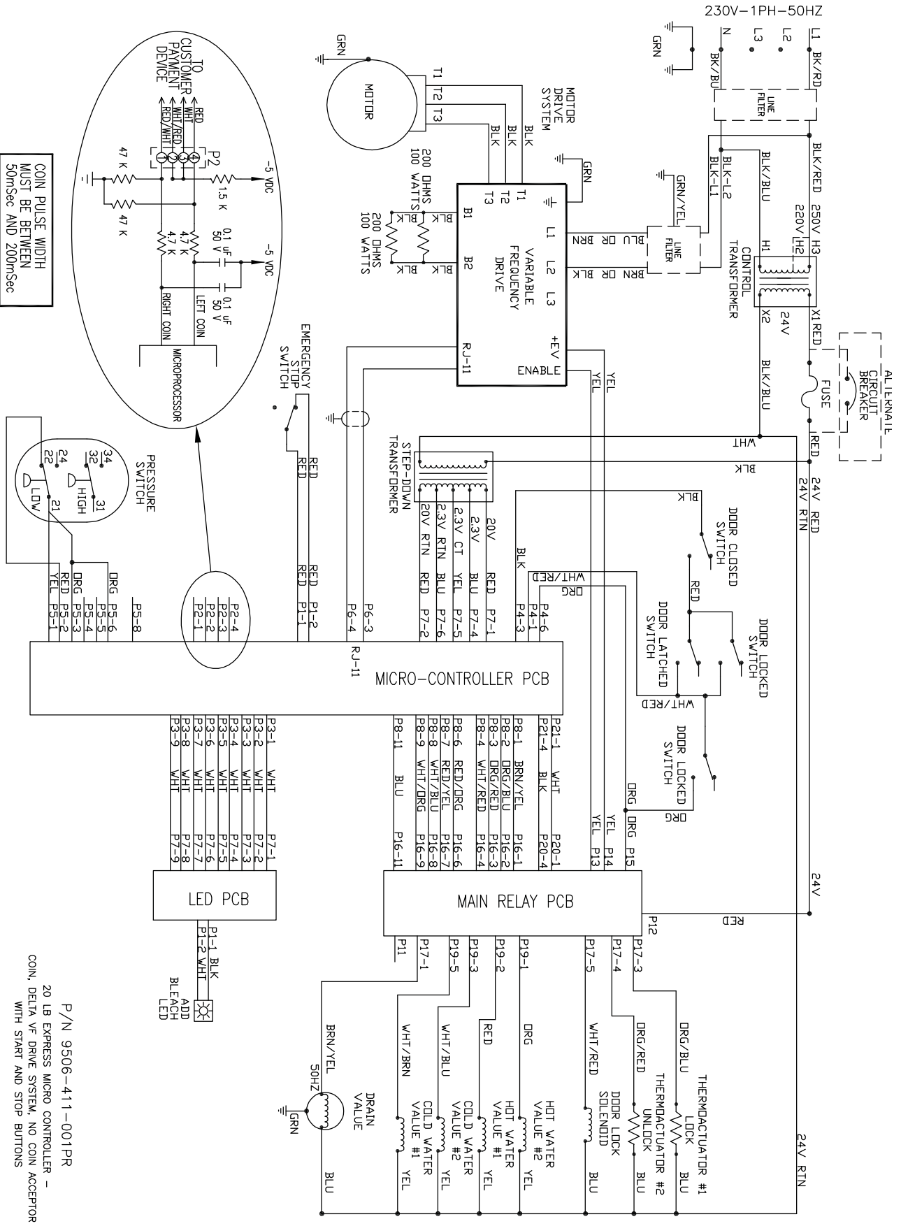
SCHEMATIC - 230V-1PH-50HZ
